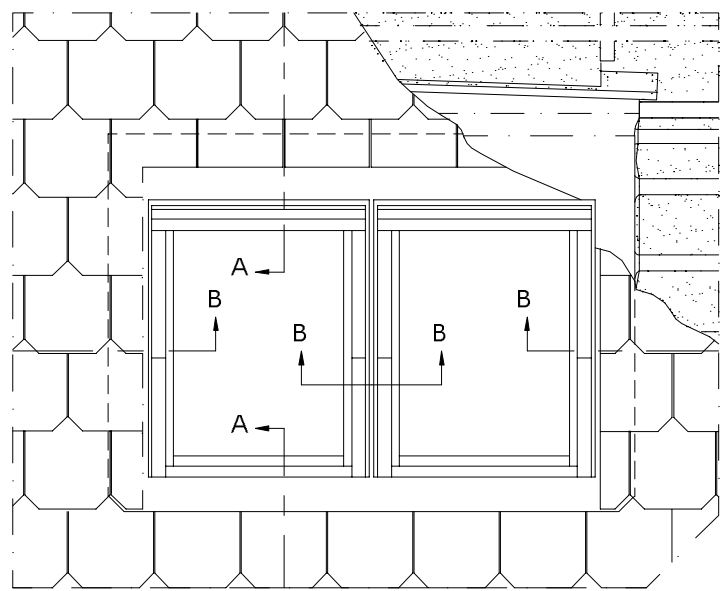
Sheer plan perpendicular to roof
