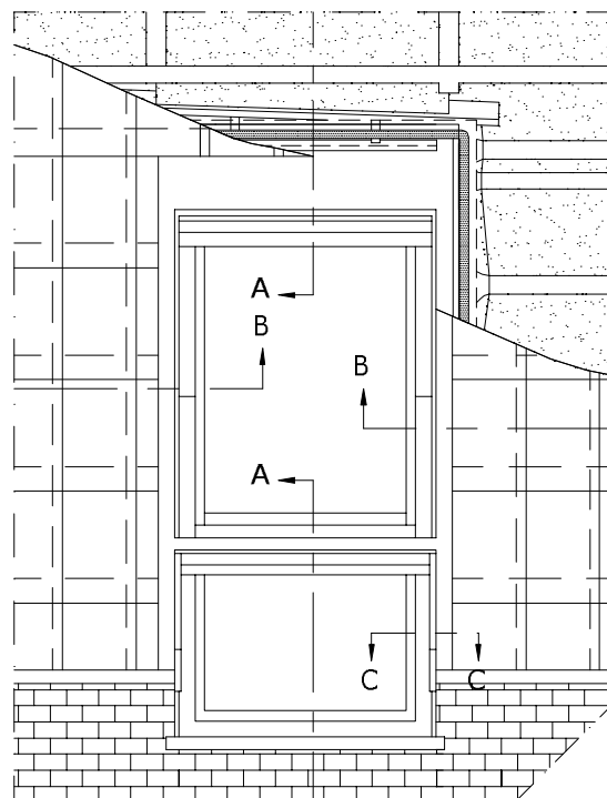
Sheer plan perpendicular to roof
