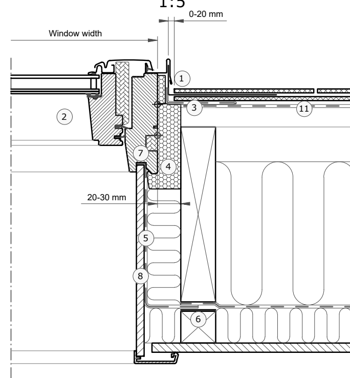
Section B-B 1:5
