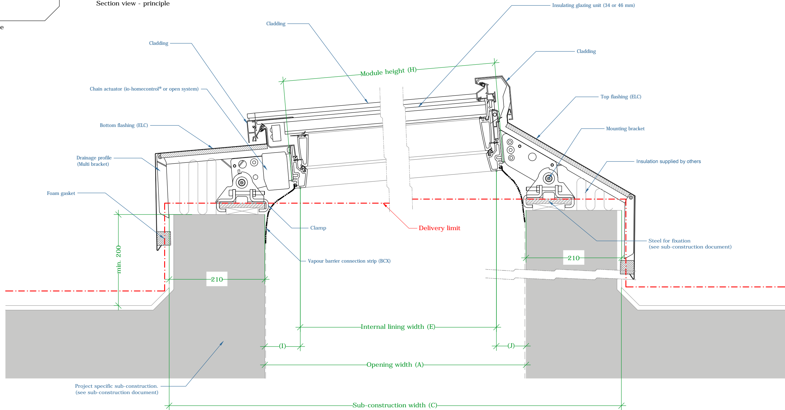
Section view - principle
