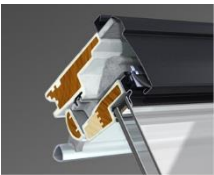
5 Excellent insulation • expanded polystyrene • colour: grey charcoal • thermally modified timber
